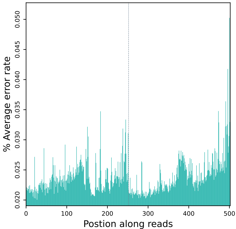
Error rate distribution along reads (CK2)
